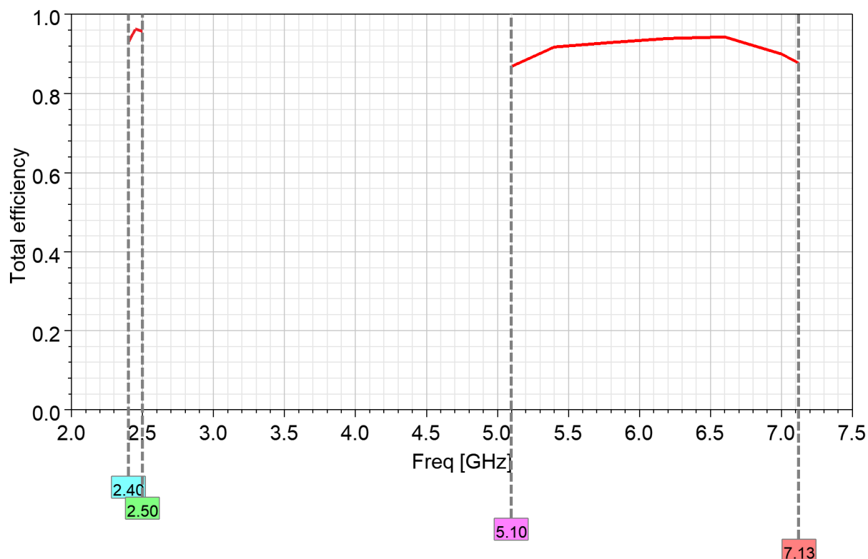
Radiation efficiency
